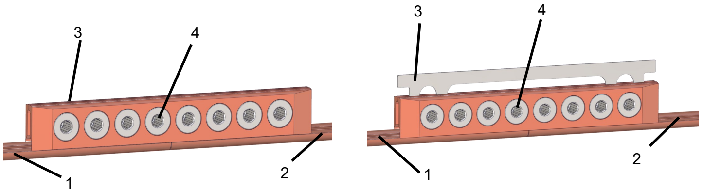
A Splice fitting for contact wire groove type AC, Contact wire groove 5.51 - 5.60 mm
